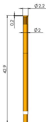
KS-215 M1,6-F-R
