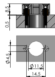
HAS-819/ HAS-819 160 (Consisting of Contact Mounting, Threaded Pins, Springs and Screws)
