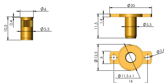
KS-410 KM5-R
