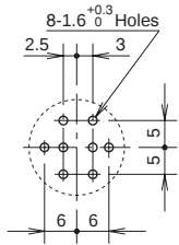
PC Board Mounting Hole Layout (Bottom View)
