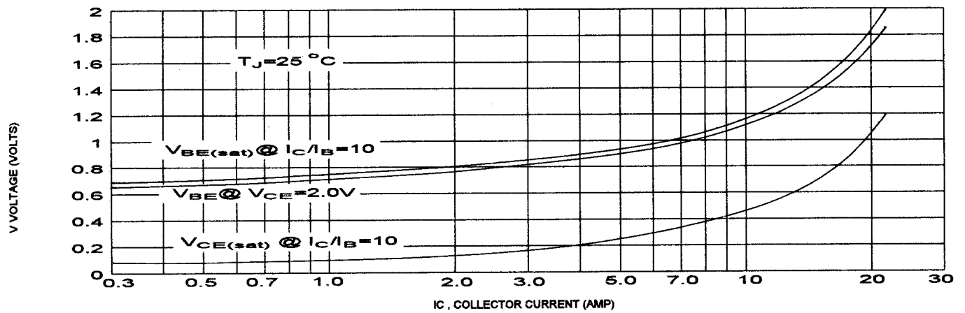
"ON" VOLTAGES
