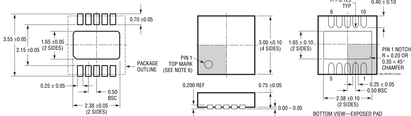
DD Package 10-Lead Plastic DFN (3mm × 3mm) (Reference LTC DWG # 05-08-1699 Rev C)
