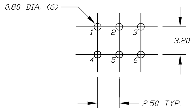
RECOMMEND P.C.B. HOLES
