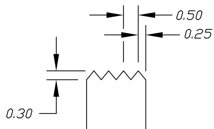
KNOB DETAIL
