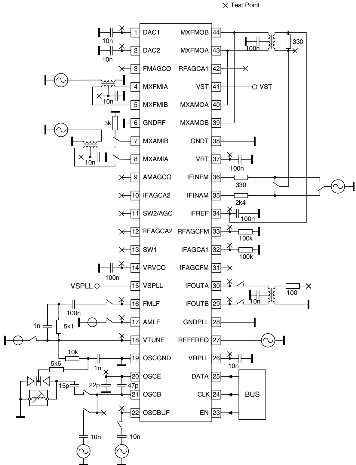
Figure 13. Test Circuit
