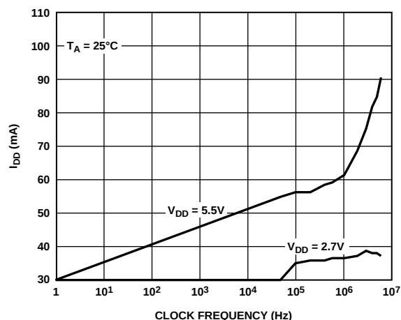
Figure 15. Supply Current vs. Clock Frequency
