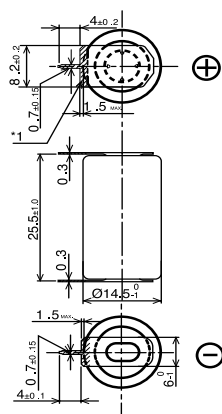
BR-1/2AAE5P
