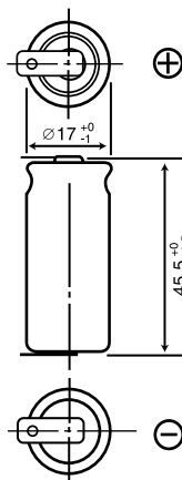
BR-AT2P BR-2/3AGT2P*
