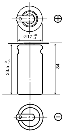
BR-2/3AT2SP BR-2/3AGT2SP*
