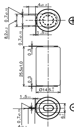
BR-1/2AAE2P
