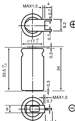
BR-2/3AE2SP BR-2/3AGE2SP*
