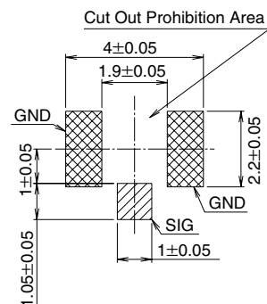
Recommended PCB mounting pattern
