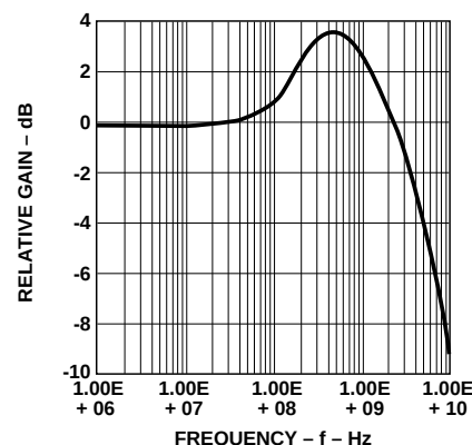
Figure 7. Typical Frequency Response Plot of the Internal Input Equalizer.
