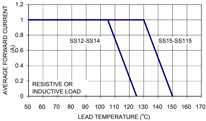
FIG.1 FORWARD CURRENT DERATING CUURVE
