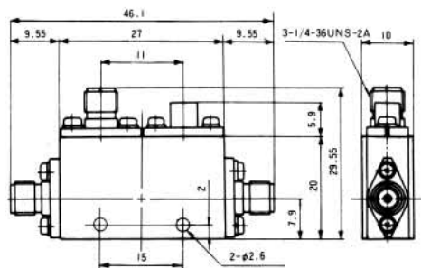
HDH-06010GID(40)
