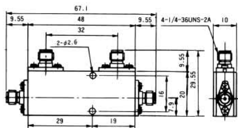
HDH-01530CI(40)
