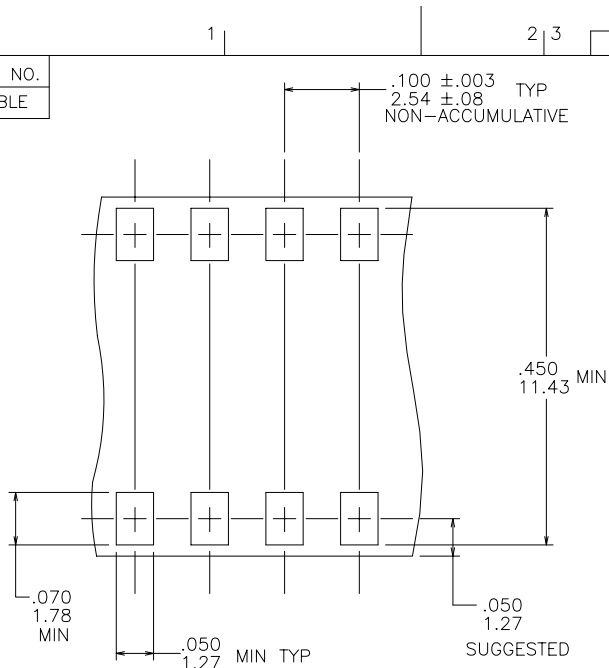
FIGURE 1 SCALE: 5:1 RECOMMENDED PCB FOOTPRINT SEE NOTE 4
