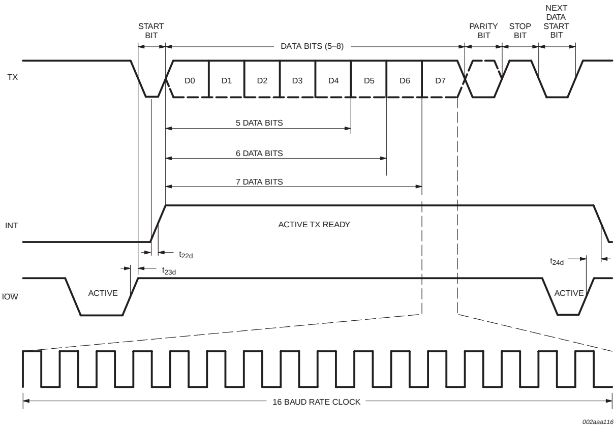
Fig 20. Transmit timing.
