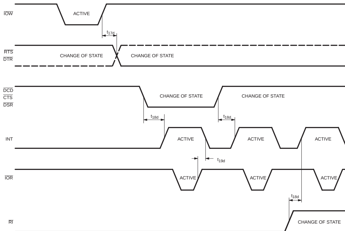
Fig 15. Modem input/output timing.
