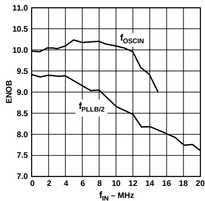
TPC 36. Rx Path ENOB vs. f_{IN}
