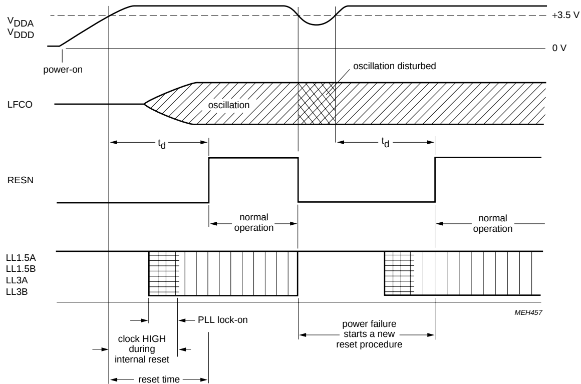
Fig.4 Reset procedure.
