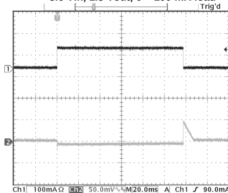
Load Transient (LDO2) 3.6 Vin, 1.8 Vout, 0 – 100 mA load
