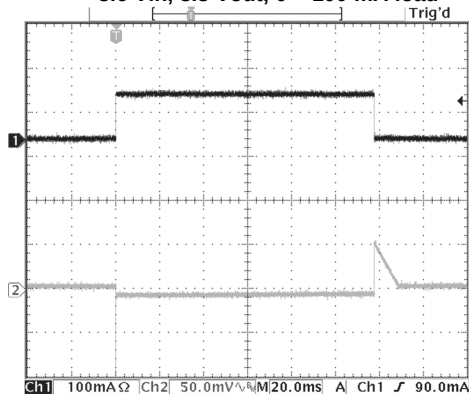
Load Transient (LDO1) 3.6 Vin, 3.3 Vout, 0 – 100 mA load
