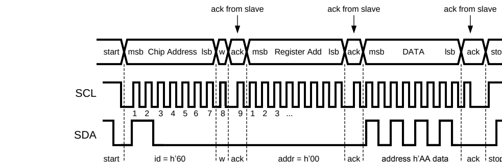
Figure 62. I 2 C Write Cycle
