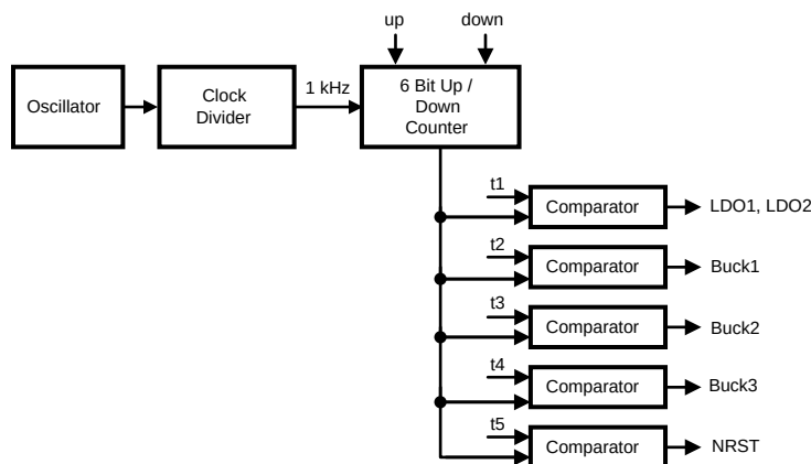
Figure 55. Power up Sequence:
