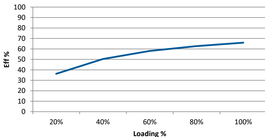
AM2F-2412SZ Efficiency vs. Loading
