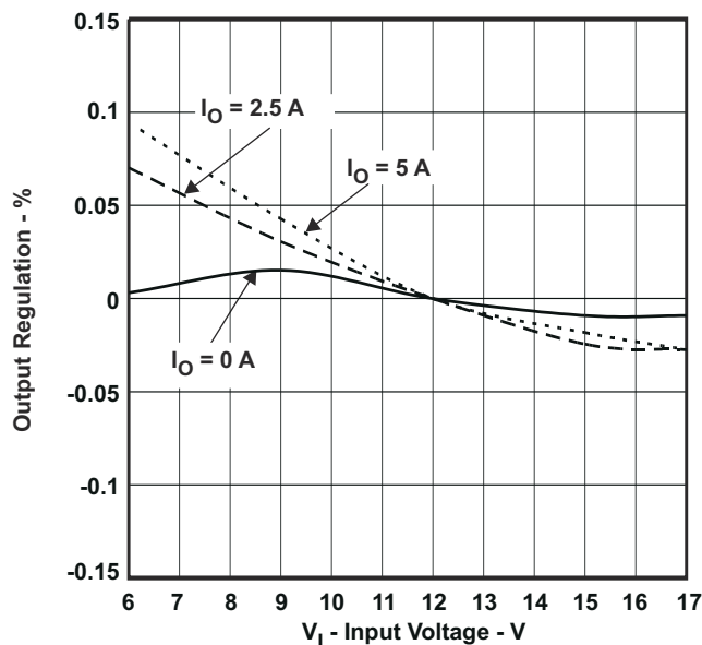
Figure 4-3. Line Regulation
