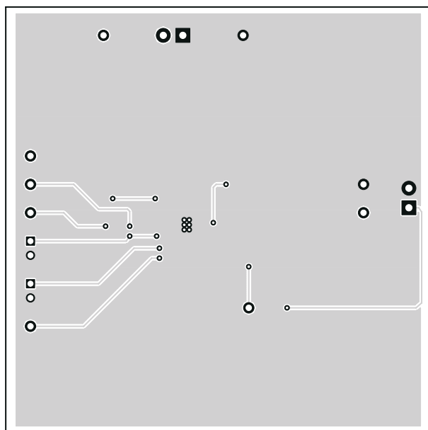
Figure 5-1. Top-Side Layout
