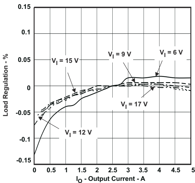
Figure 4-2. Load Regulation
