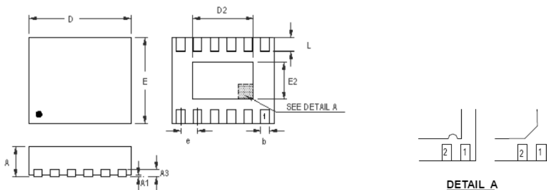
Pin #1 ID and Tie Bar Mark Options
