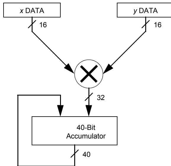
Figure 21. Multiply-Accumulator Block Diagram
