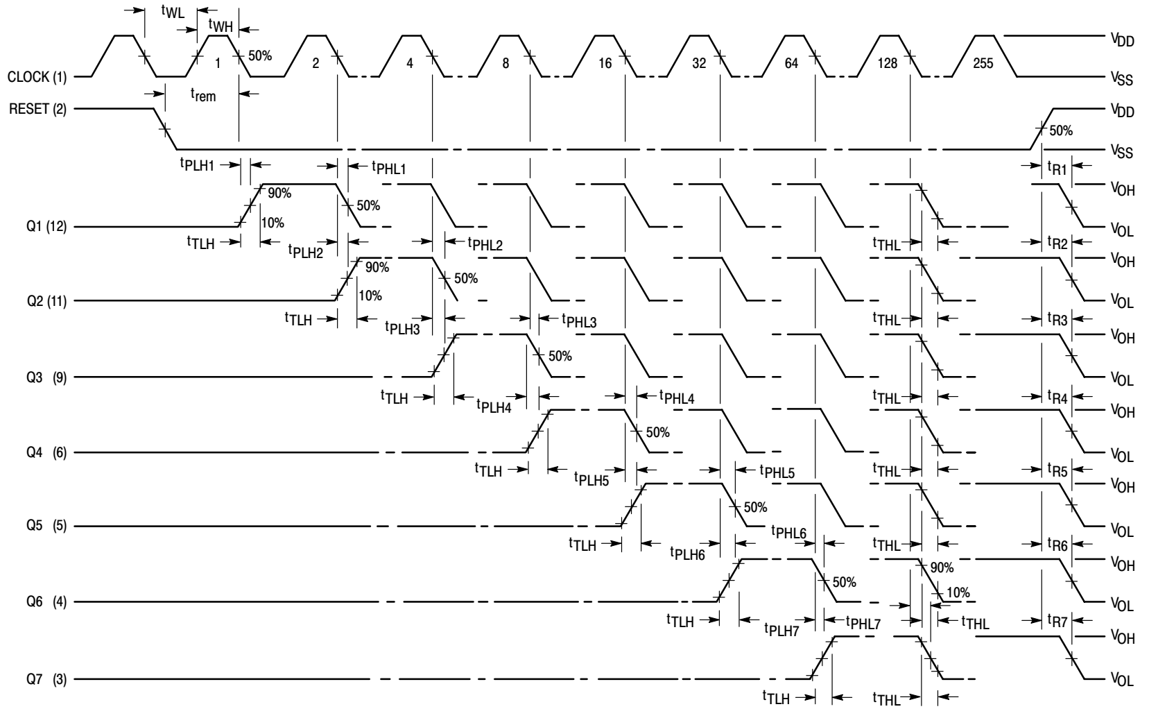
Figure 4. Functional Waveforms
