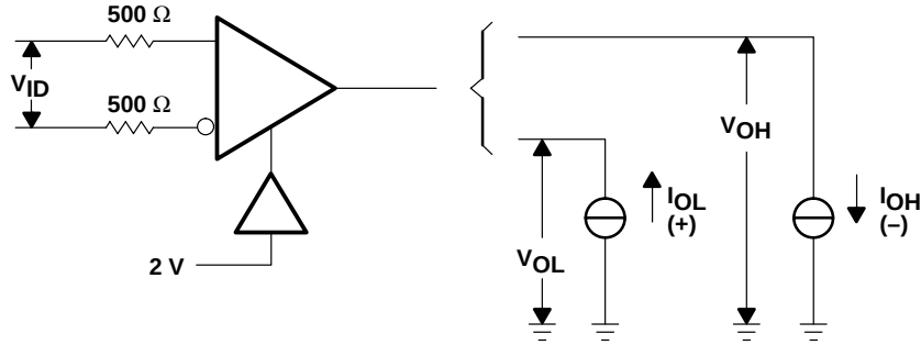
Figure 1. V_{OH} , V_{OL}
