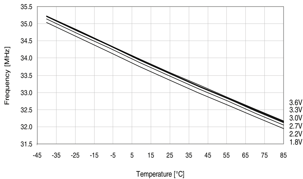
Figure 33-277. 32MHz internal oscillator frequency vs. temperature. DPLL disabled.
