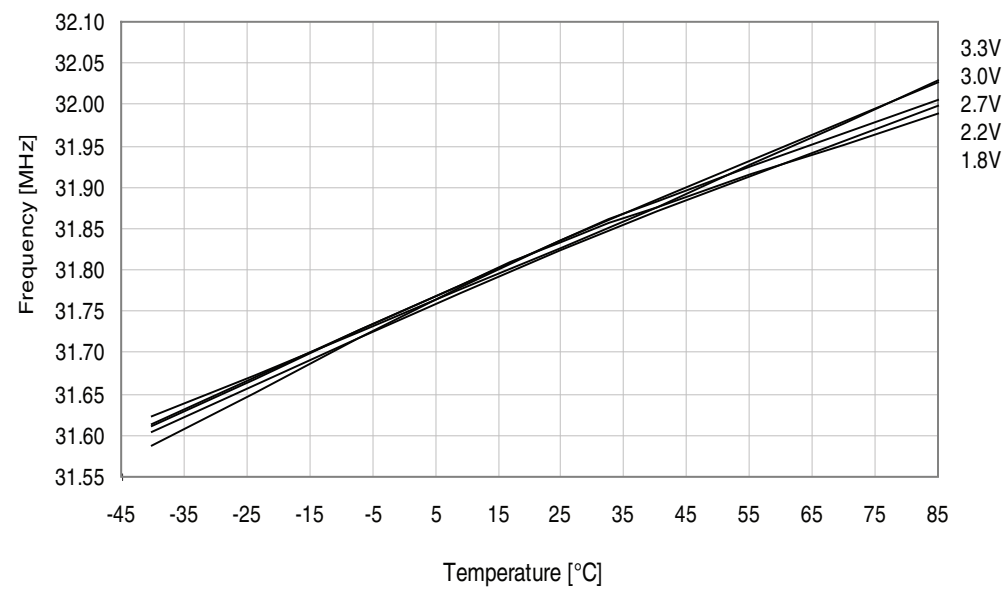
Figure 33-278. 32MHz internal oscillator frequency vs. temperature. DPLL enabled, from the 32.768kHz internal oscillator.
