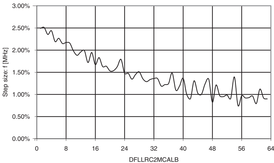
Figure 33-36. Internal 2MHz oscillator CALB calibration step size. T = -40 to 85^{\circ}\text{C} , V_{CC} = 3\text{V} .
