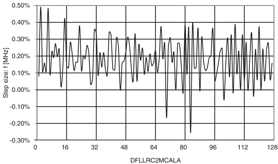
Figure 33-35. Internal 2MHz oscillator CALA calibration step size. T = -40 to 85^{\circ}\text{C} , V_{CC} = 3\text{V} .
