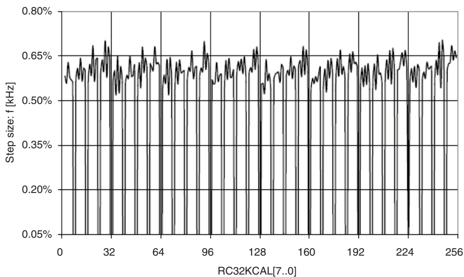
Figure 33-34. Internal 32.768kHz oscillator calibration step size. T = -40 to 85^{\circ}\text{C} , V_{CC} = 3\text{V} .
