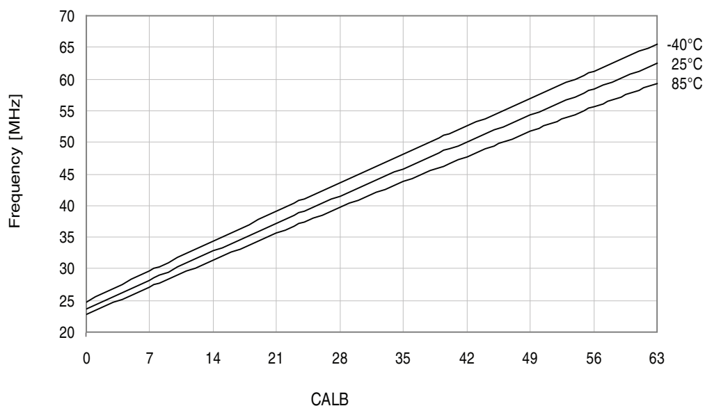
Figure 33-213. 32MHz internal oscillator frequency vs. CALB calibration value. V_{CC} = 3.0V .
