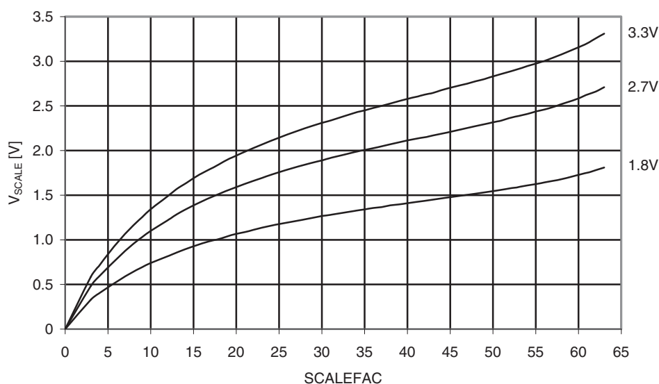
Figure 34-5. Analog comparator voltage scaler vs. scalefac.
