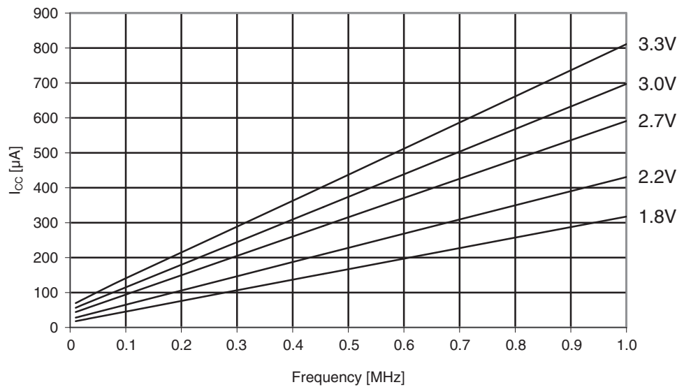
Figure 33-1. Active supply current vs. frequency. f_{SYS} = 0 - 1\text{MHz} external clock, T = 25^{\circ}\text{C} .
