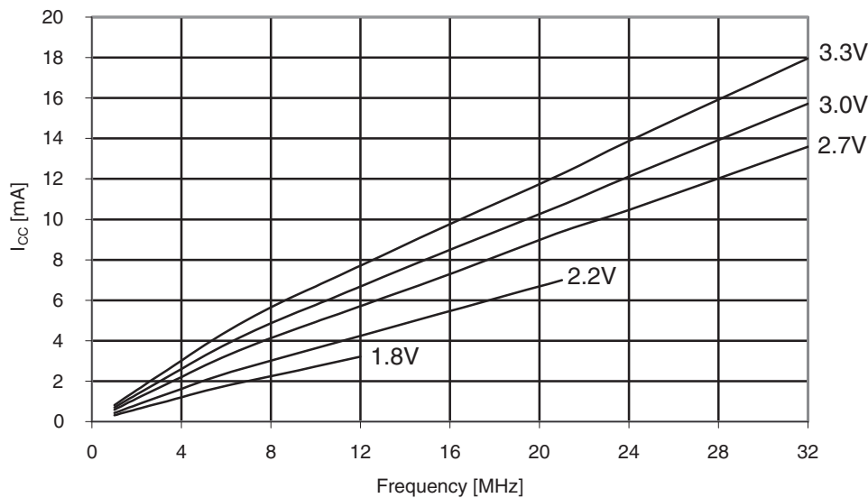
Figure 33-2. Active supply current vs. frequency. f_{SYS} = 1 - 32\text{MHz} external clock, T = 25^{\circ}\text{C} .
