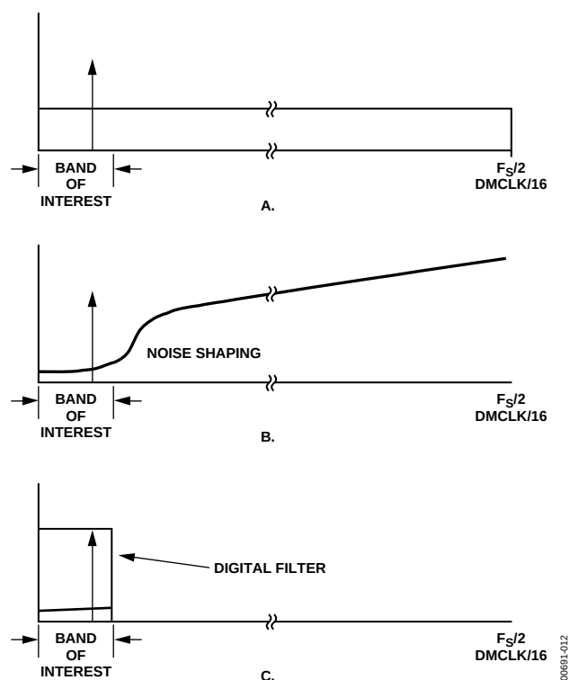
Figure 12. Sigma-Delta Noise Reduction
