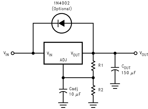
FIGURE 5. Regulator with Protection Diode
