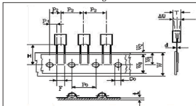
Fig.1 P=5.0、7.5mm
