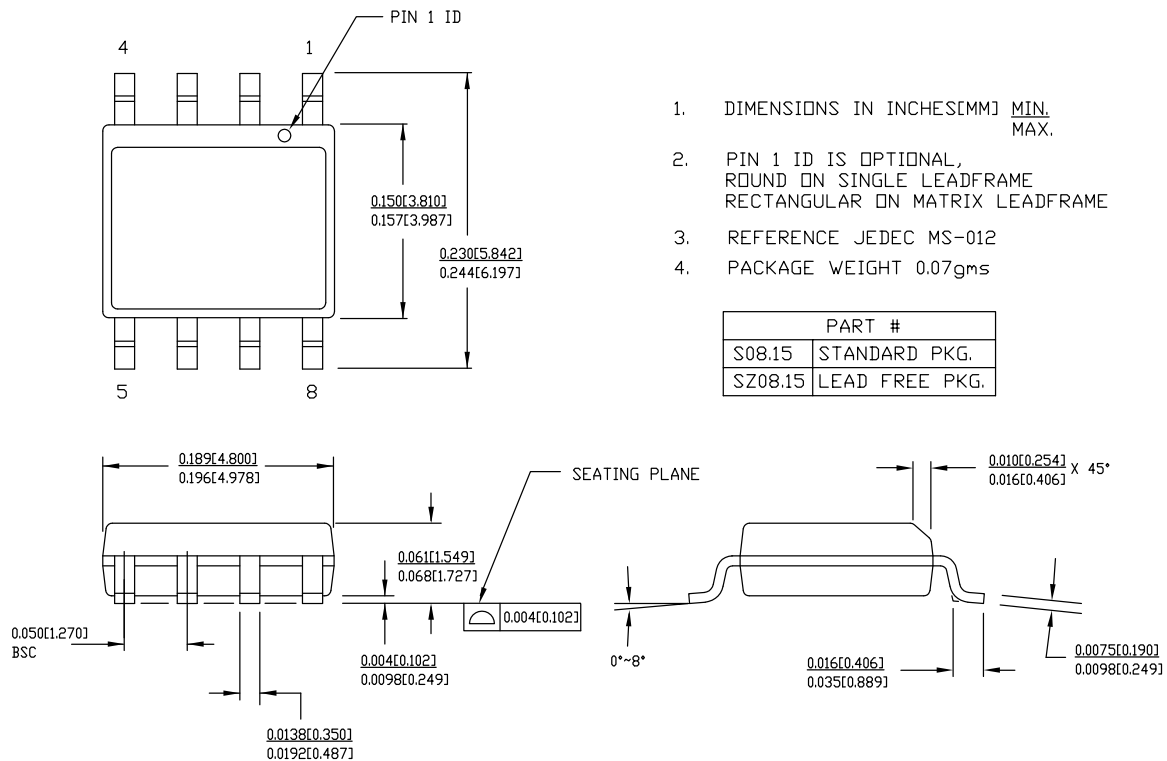
Figure 7. 8-pin SOIC (150-Mils) S08.15/SZ08.15
