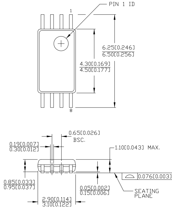
Figure 7. 8-pin TSSOP (4.40 mm Body) Z08.173/ZZ08.173
