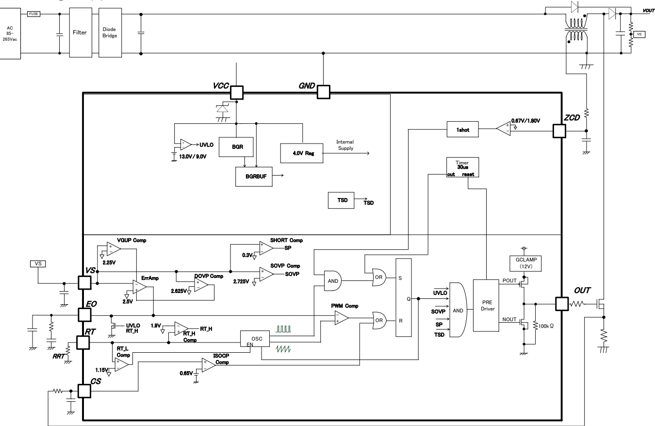
Figure 3. Block Diagram
