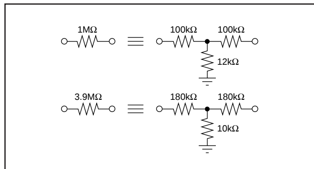
FIGURE 6. Equivalent Resistances.
