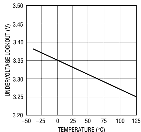
Undervoltage Lockout vs Temperature (Controller)
