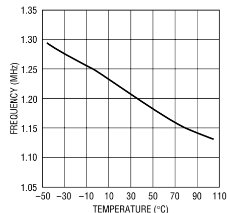
Auxillary Regulator Switch Oscillator Frequency
