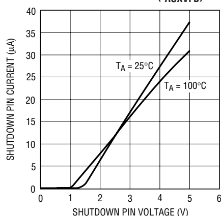
Shutdown Pin Current ( I_{\text{AUXVFB}} )
