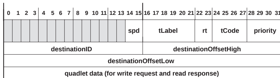
Figure 5–1. Quadlet-Transmit Format
