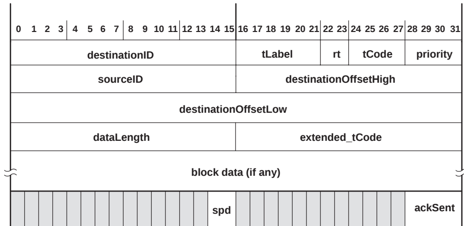
Figure 5–4. Block-Receive Format
