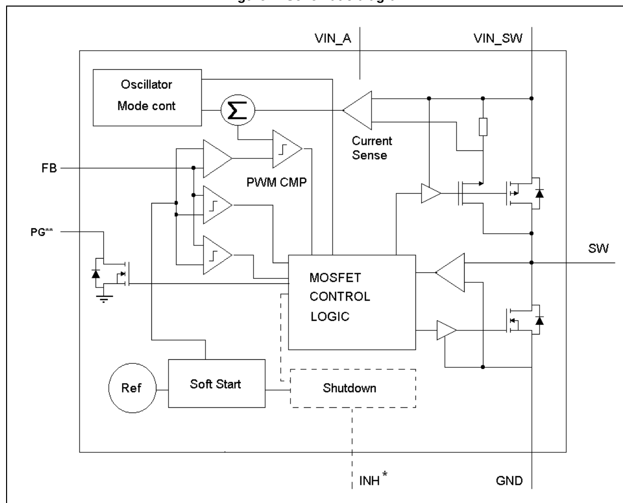
Figure 1. Schematic diagram
