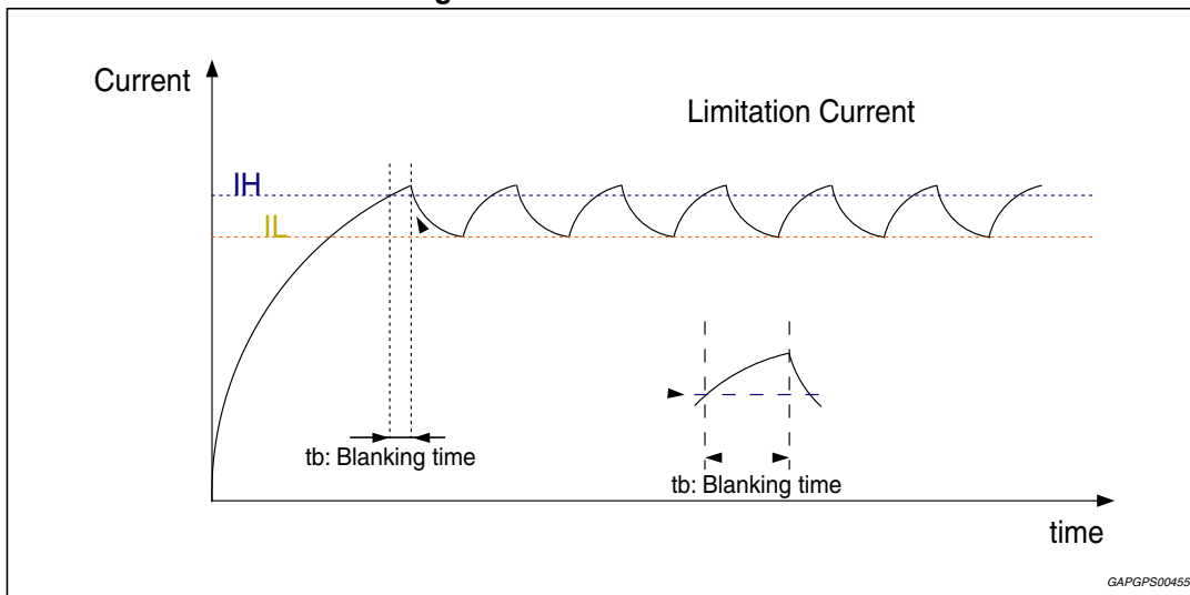
Figure 11. Current limitation
