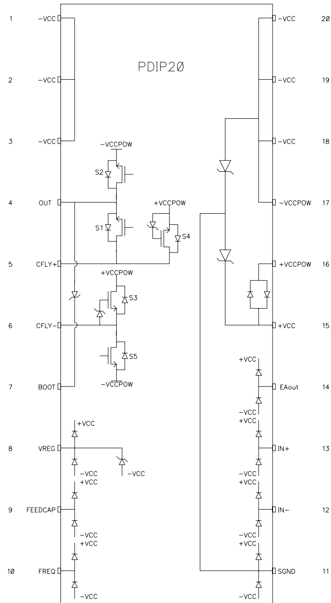
Figure 8: ESD Protection Structure
