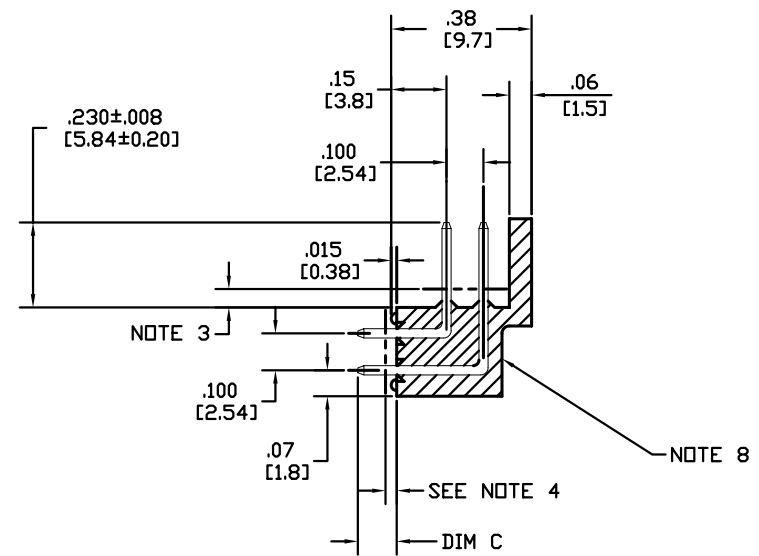
SECTION Z-Z
