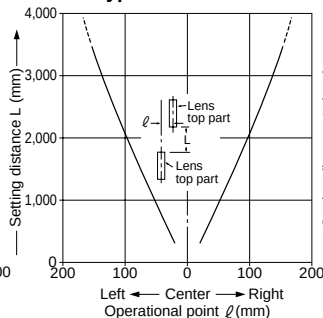
FT-FM2 Thru-beam
