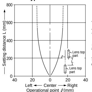
FT-R80 Thru-beam
