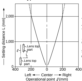
FT-P80 Thru-beam
