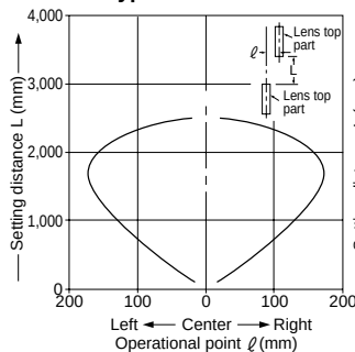
FT-C4 Thru-beam
