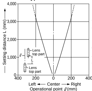
FT-B8 Thru-beam
