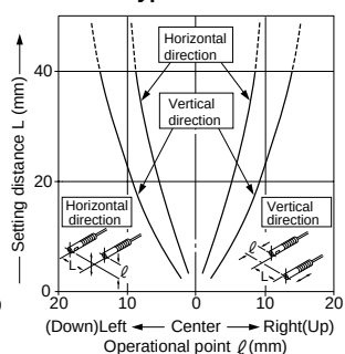
FT-P80 Thru-beam
