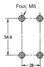
Mounting Dimensions
