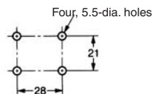
Bottom Mounting
