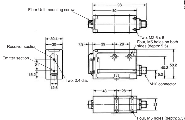
Bottom Mounting
