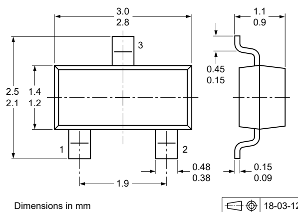
Fig. 11. Package outline SOT23 (TO-236AB)
