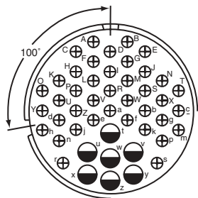
100° Rotation of 36-7 36-16
