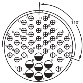
110° Rotation of 36-7 36-17
