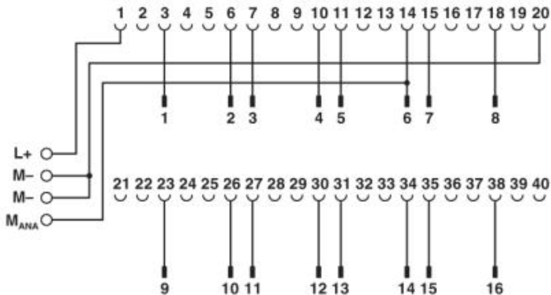
Connection scheme FLKM 16-PA-332-5HF//MINI-MCR
