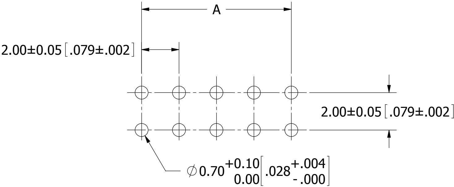
RECOMMENDED PCB LAYOUT P.C. BOARD THICKNESS: 1.6mm[.063"]
