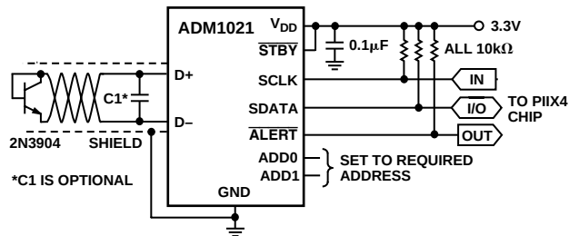
Figure 18. Typical ADM1021 Application Circuit
