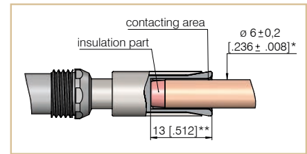
Example of contacting with HKR-612 600 ... M, Ø 6 mm
