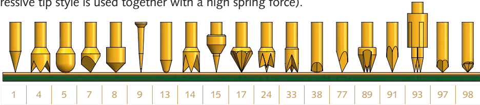
Most commonly used tip styles
