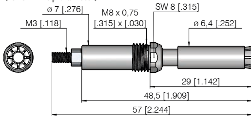
HKR-612 400 100 S 10003 M (for 4 mm tip diameter)
