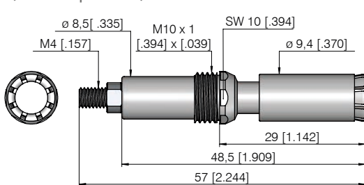
HKR-612 600 130 S 20003 M (for 6 mm tip diameter)
