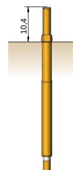
DPS-465...02 M with KS-465 M2,5
