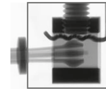
Example: Contacting of a print clip with T-785 M
