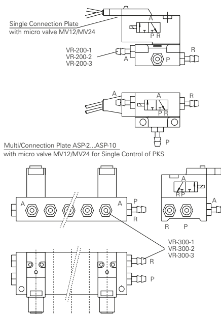
Ordering examples to activate and control 5 PKS-300
