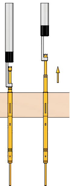
Install and remove GKS in KS (head- \varnothing > plunger shaft- \varnothing )
