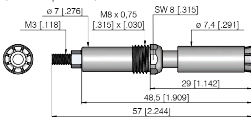
HKR-612 600 130 S 20003 M (for 6 mm tip diameter)
