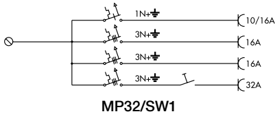
Wiring diagram
