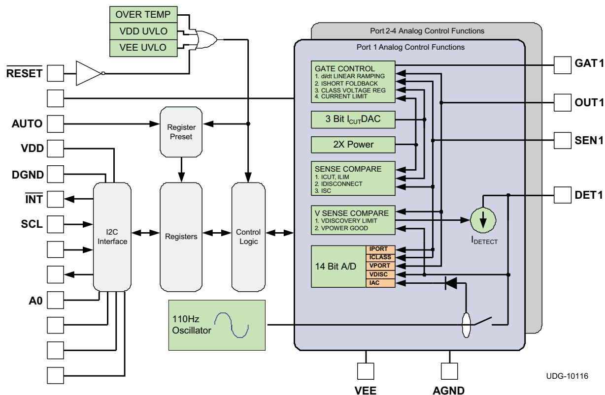
Figure 24. Block Diagram
