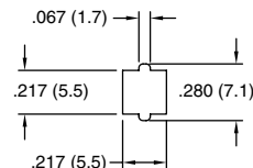
Mounting Hole
