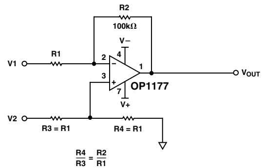
Figure 13. Difference Amplifier
