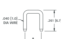
SHORTING PIN
