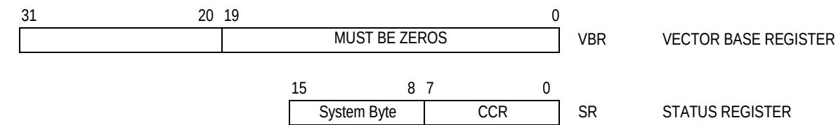
Figure 3-4. Supervisor Programming Model
